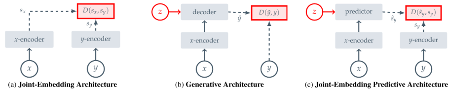
Figure 3.4 Three SSL prediction paradigms: joint-embedding (a), generative (b), and joint-embedding predictive (c) [14].
