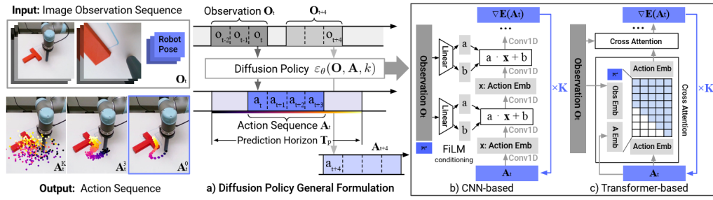
Figure 3.3 Diffusion Policy: general formulation (a), CNN variant (b), transformer variant (c) [9].
