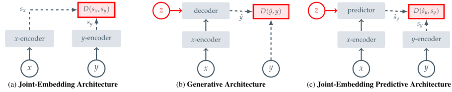
Figure 3.7 Three SSL prediction paradigms: joint-embedding (a), generative (b), and joint-embedding predictive (c) [14].
