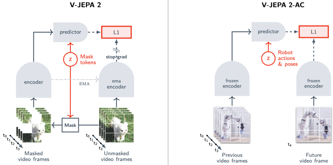
Figure 3.9 Standard V-JEPA2 (left) versus action-conditioned V-JEPA2-AC (right) [24].
