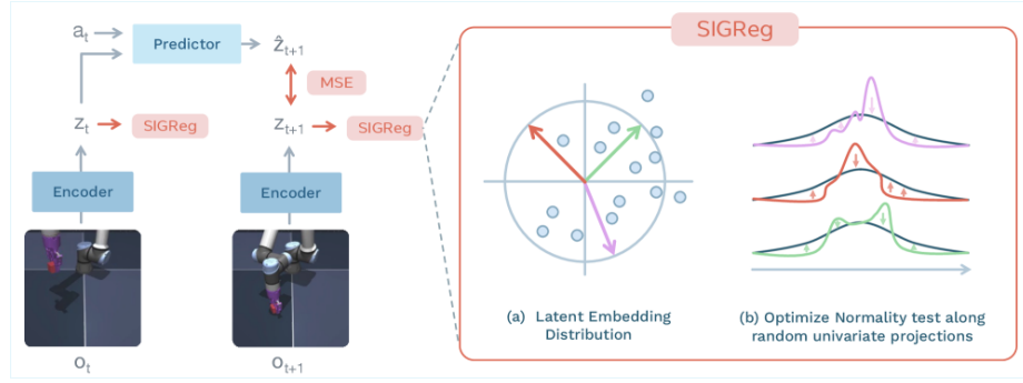
Figure 3.11 LeWM training pipeline: encoder, dynamics predictor, and SIGReg regulariser [26].
