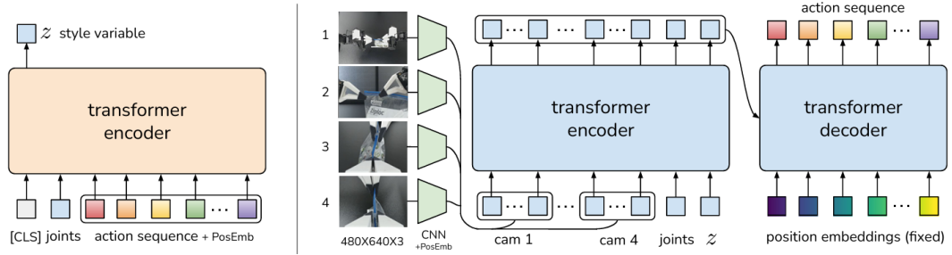
Figure 3.2 Architecture of the Action Chunking with Transformers (ACT) policy [8].
