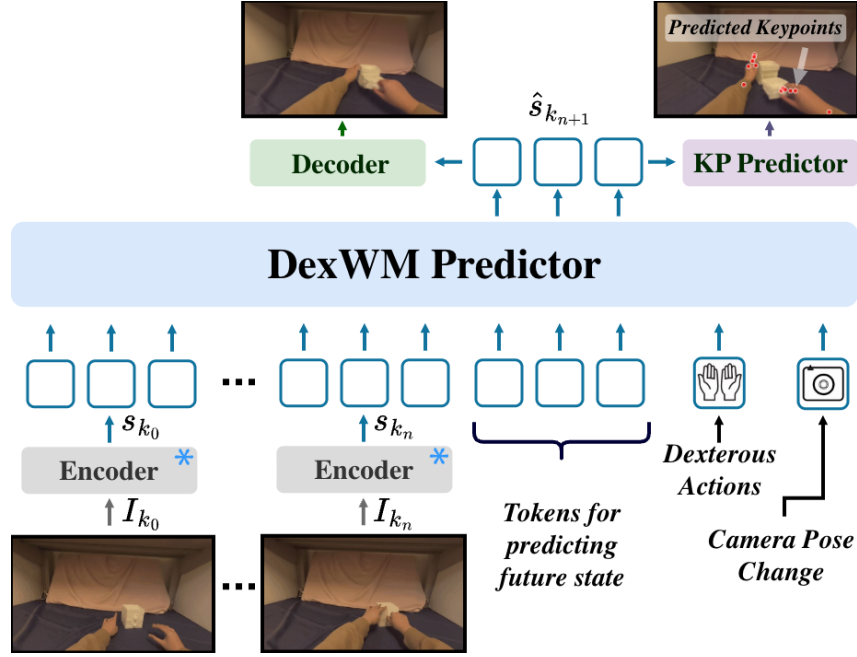
Figure 3.10 High-level layout of the DexWM world model pipeline, illustrating how predicted keypoints are incorporated alongside the encoder, CDiT predictor, and decoder stages [25].
