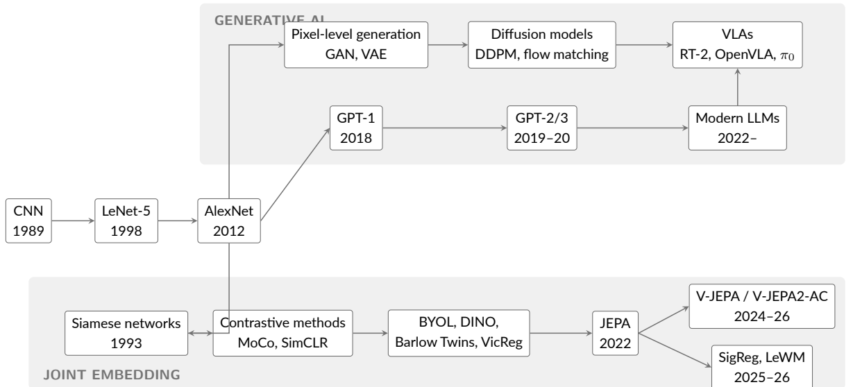
Figure 3.4 The post-AlexNet split of visual representation learning into a generative branch, culminating in diffusion models and the VLAs debated above, and a joint-embedding branch, culminating in JEPA-style latent world models including the families evaluated in this benchmark. Adapted from [41].
