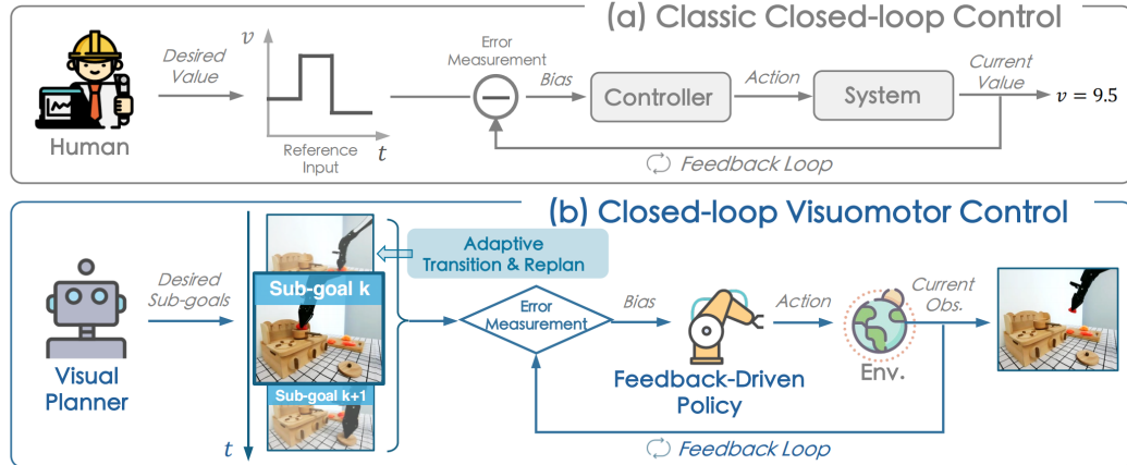
Figure 3.6 Classic closed-loop control (a) versus CLOVER’s closed-loop visuomotor control (b) [44].
