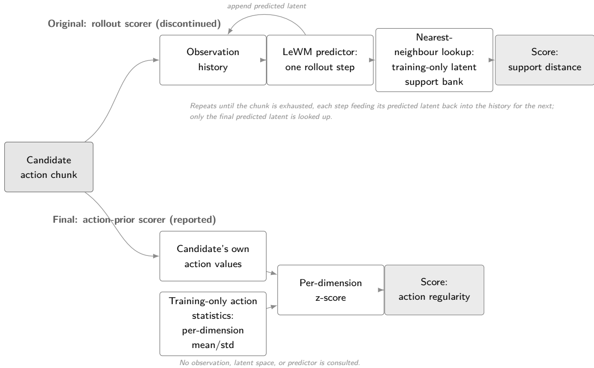
Figure 5.7 The two LeWM scoring routes implemented in this study, starting from the same candidate action chunk. The original rollout scorer (top) autoregressively rolls the candidate forward through the LeWM predictor, feeding each predicted latent back into the observation history for the next step, then looks up the final predicted latent’s nearest neighbour in a training-only latent support bank. The final action-prior scorer (bottom, the route reported as a result) skips visual rollout entirely and scores the candidate’s own action values directly against training-only action statistics.
