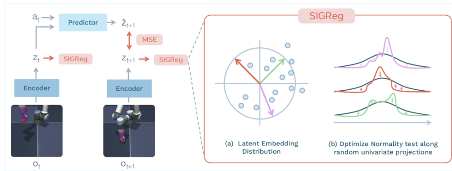
Figure 3.10 LeWM training pipeline: encoder, dynamics predictor, and SIGReg regulariser [26].
