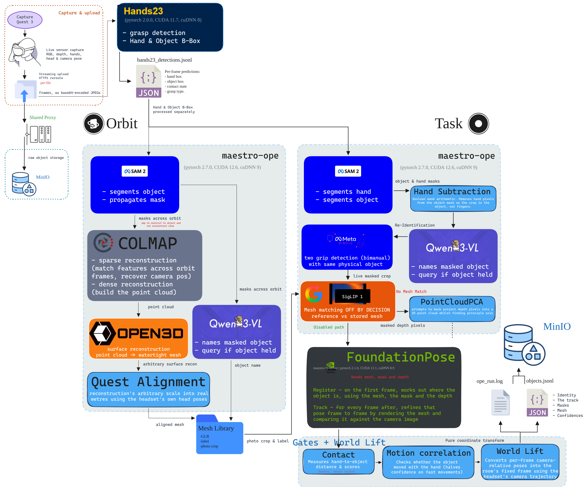
Figure 1. Refined Maestro VR pipeline, preserved from the supplied audit assets. Arrows describe architectural relationships, including conditional and disabled paths. The October 3 hand-distance guard is documented below and is not drawn in this earlier diagram.
