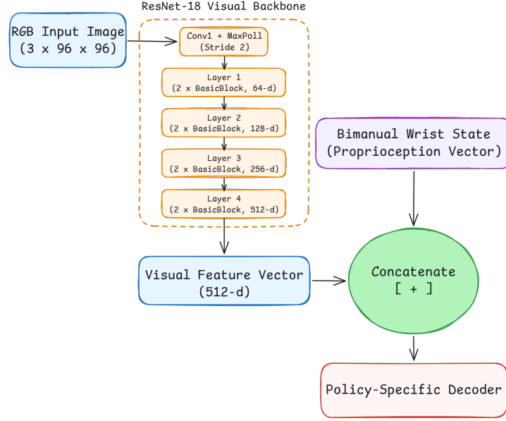
Figure 5.1 Shared ResNet-18 visual backbone preceding both policy decoders. Adapted from [60].
