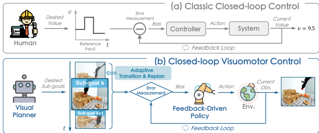
Figure 3.3 Classic closed-loop control (a) versus CLOVER’s closed-loop visuomotor control (b) [35].
