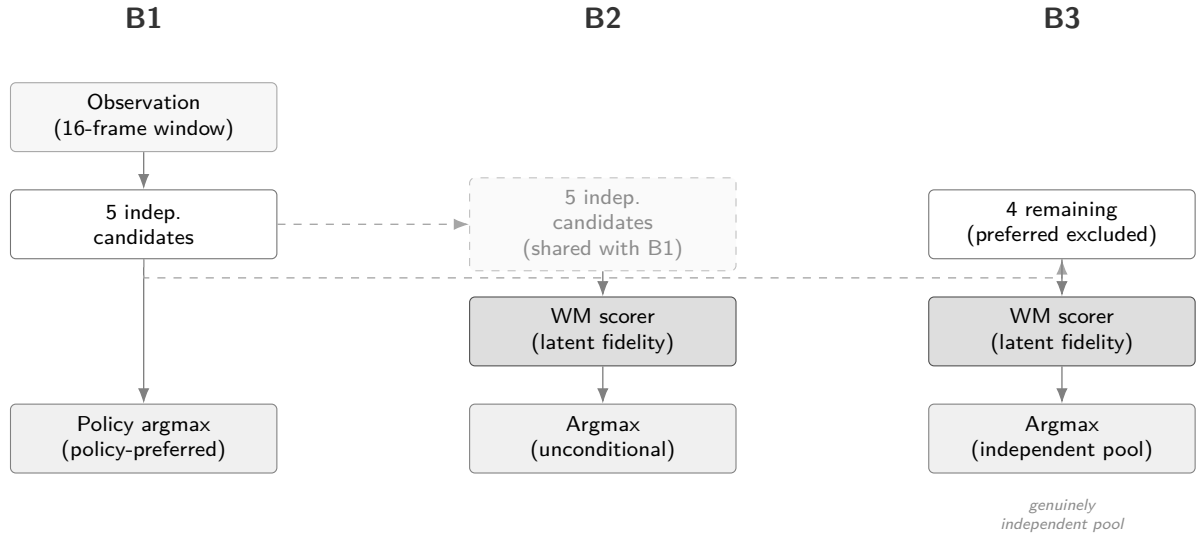
Figure 4.3 Three-branch evaluation framework (Section 4.2), shown for a policy producing five independent candidates. B2 and B3 reuse the same candidate pool generated for B1 (dashed lines) rather than regenerating it; B3 additionally removes the policy’s preferred candidate before scoring. Both ACT and DP follow this design; the per-policy candidate-generation mechanics are detailed in Section 4.3.
