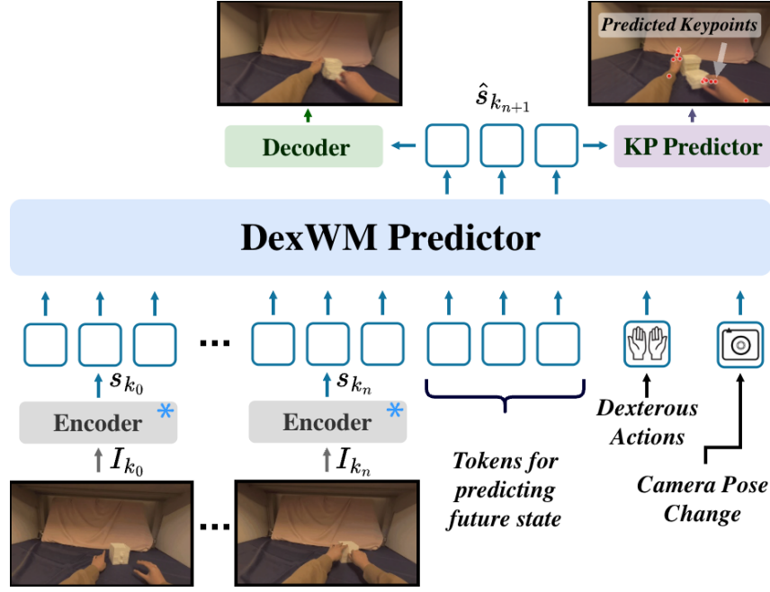
Figure 3.7 High-level layout of the DexWM world model pipeline, illustrating how predicted keypoints are incorporated alongside the encoder, CDiT predictor, and decoder stages [30].
