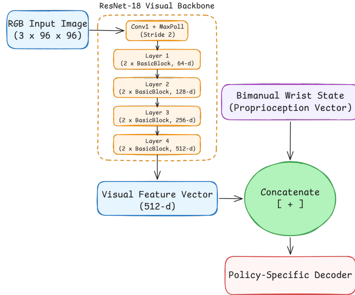
Figure 5.3 Shared ResNet-18 visual backbone preceding both policy decoders. Adapted from [56].
