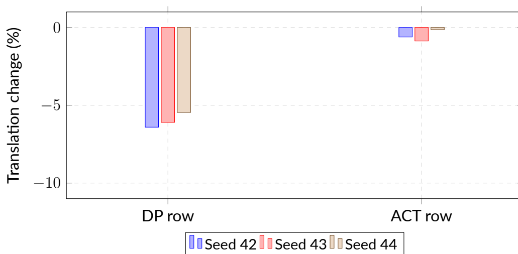
Figure 6.2 V-JEPA2-AC’s Branch 2 translation change across three training seeds, DP row and ACT row. Level bars indicate a stable result; the DP row’s three bars sit close together, confirming the headline result is not a single-run artefact.
