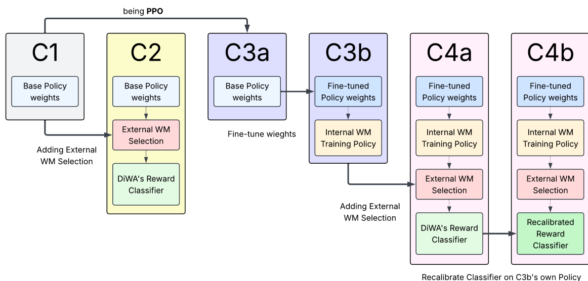
Figure 6.3 How the six conditions relate. Arrows show which checkpoint each condition starts from and what changes on the way to it. DiWA's policy, world model, and reward classifier are the same three modules used throughout this section; only their role changes between conditions.
