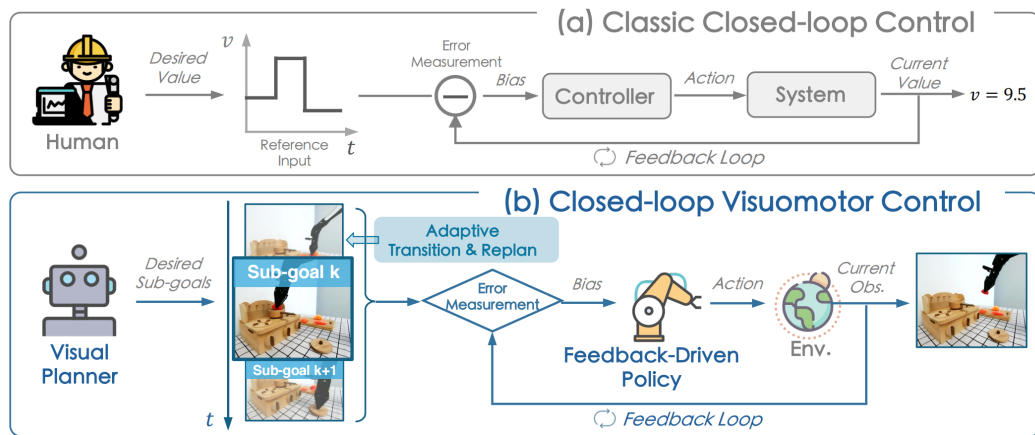
Figure 3.3 Classic closed-loop control (a) versus CLOVER’s closed-loop visuomotor control (b) [31].
