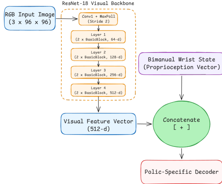
Figure 5.1 Shared ResNet-18 visual backbone preceding both policy decoders. Adapted from [46].
