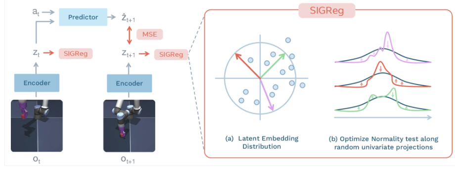
Figure 3.8 LeWM training pipeline: encoder, dynamics predictor, and SIGReg regulariser [33].
