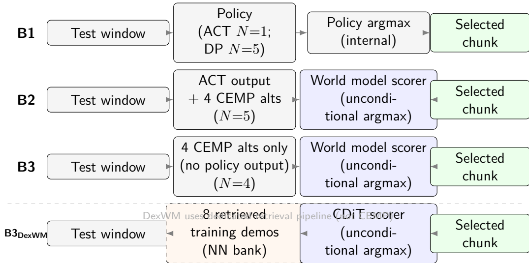
Figure 5.4 Guard evaluation pipeline for all branches. B2 pools include the ACT output alongside four CEMP-planned alternatives; B3 pools contain the four CEMP alternatives only, with the policy output excluded. The DexWM B3 variant (dashed border) uses a distinct pipeline in which eight retrieved training demonstrations replace the CEMP pool; see Section 5.8.
