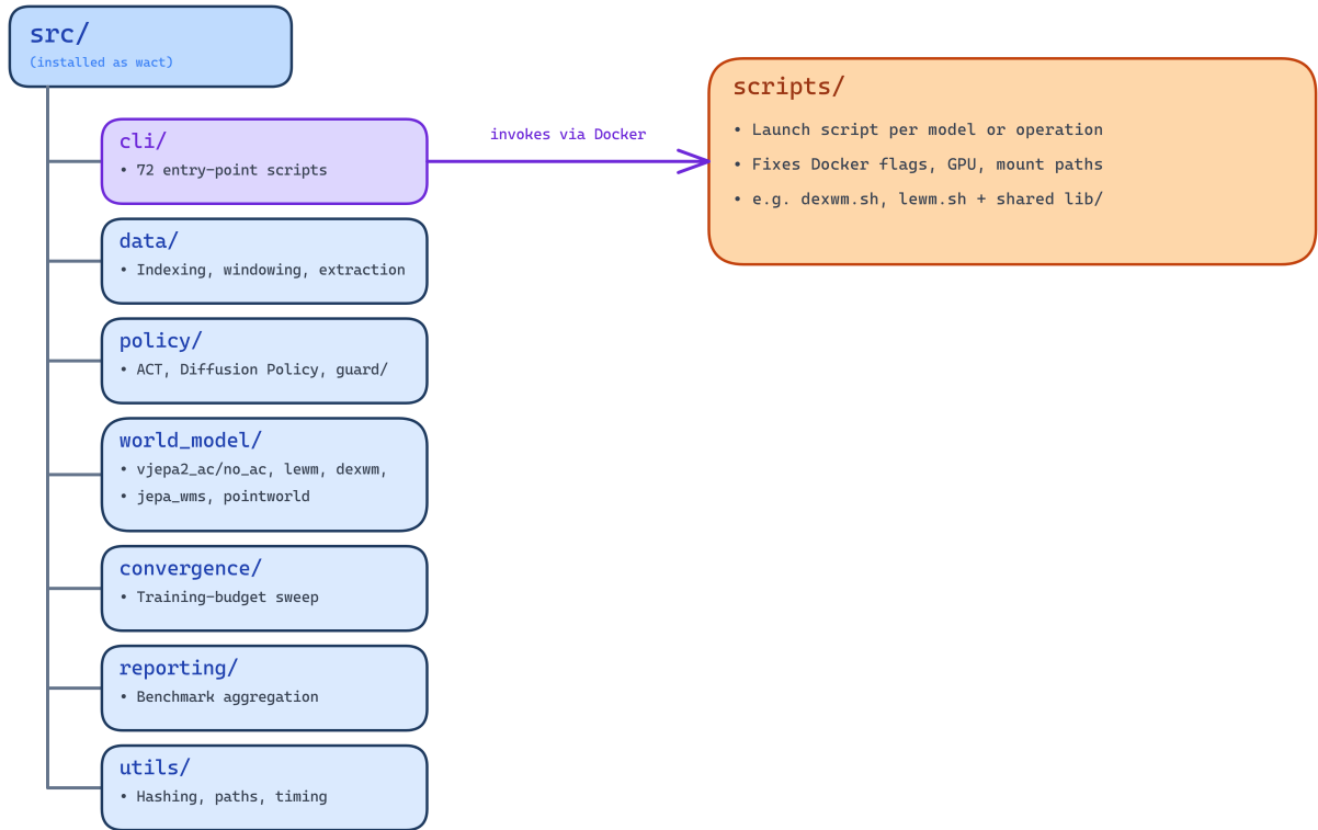
Figure 5.1 Package structure under src/ , and how scripts/ launches cli/ entry points inside Docker. policy/guard and every world_model/ submodule implement the scoring interface used by the guard evaluation of Section 5.8.
