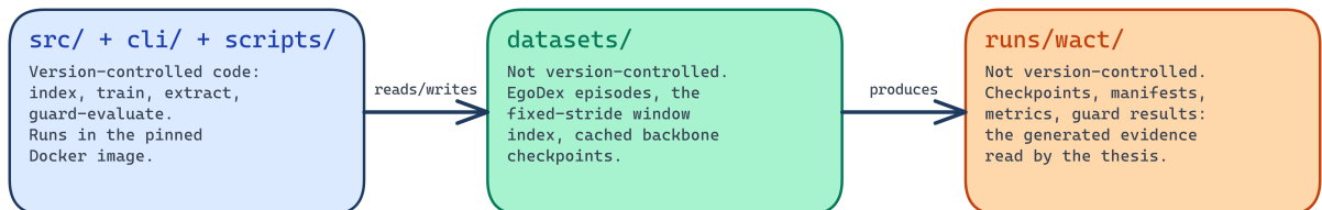
Figure 5.2 Data flow between the version-controlled code ( src/ , cli/ , scripts/ ) and the generated, non-version-controlled artefacts ( datasets/ , runs/wact/ ). All three stages execute inside the same pinned Docker image; only the code is tracked by git, keeping the audit trail between code and generated evidence unambiguous.
