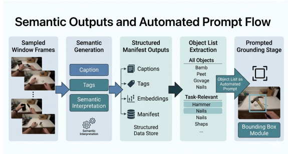
Figure 2: Example object-list prompt source emitted by the semantic stage. The same structured object field is reused as input for the grounding stage.
