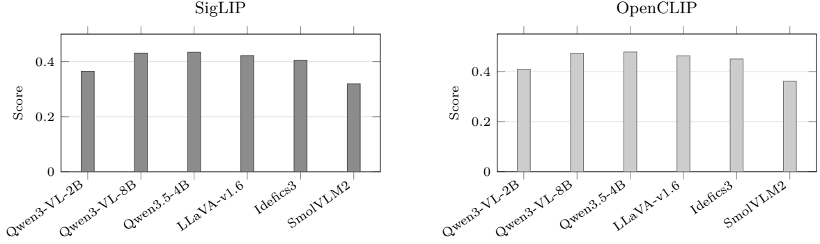
Figure 4: Semantic benchmark score distributions over the shared 64-window sample. SigLIP and OpenCLIP are plotted separately because their cosine similarity values are calibrated within different embedding spaces.
