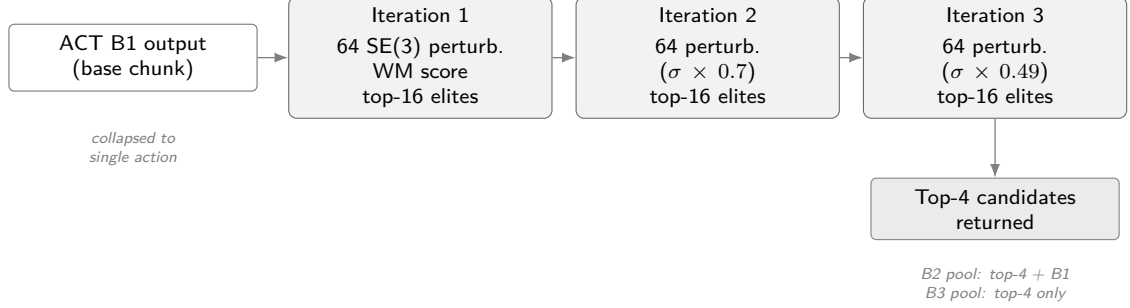
Figure 4.3 CEMP candidate augmentation for ACT-based guards. Three optimisation iterations refine perturbations around the policy’s collapsed output; the standard deviation decays by 0.7\times per iteration. The four highest-scoring candidates across iterations form the B2/B3 evaluation pool.
