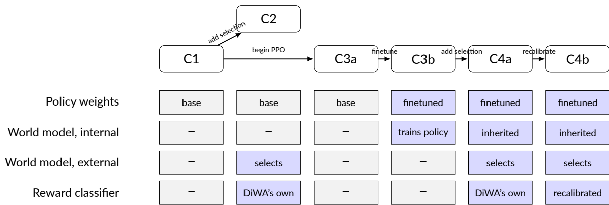
Figure 6.2 How the six conditions relate. Arrows show which checkpoint each condition starts from. Shaded cells mark where a module is active for that condition; DiWA's policy, world model, and reward classifier are the same three modules used throughout this section, only their role changes.
