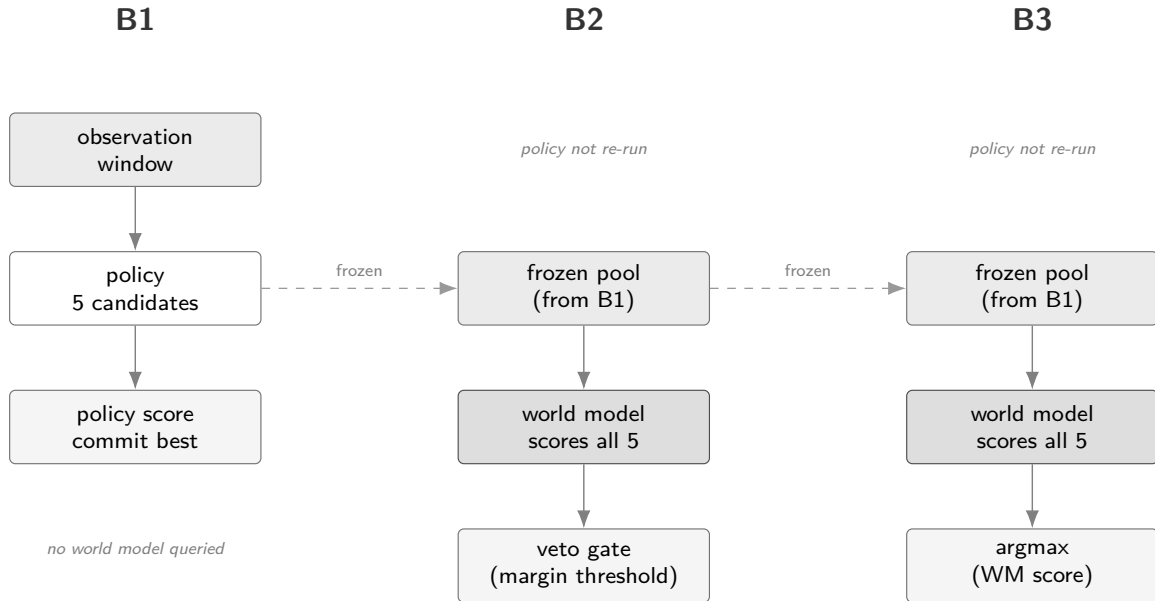
Figure 4.3 Three-branch design space for V-JEPA2-AC, V-JEPA2 no-AC, LeWM, and PointWorld. B1 generates the candidate pool and uses the policy’s own preference alone; B2 adds a world-model veto constrained by a margin threshold; B3 gives the world model full selection authority over the same frozen pool produced at B1 time. The policy is not re-run in B2 or B3. DexWM uses a distinct B3 design in which the frozen pool is replaced by eight training demonstrations retrieved from the training bank; see text.
