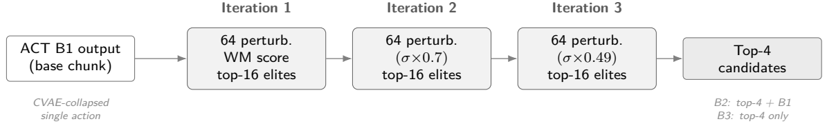
Figure 5.5 CEMP candidate augmentation, refining SE(3) perturbations of the ACT B1 output over three iterations to form the B2/B3 evaluation pool.
