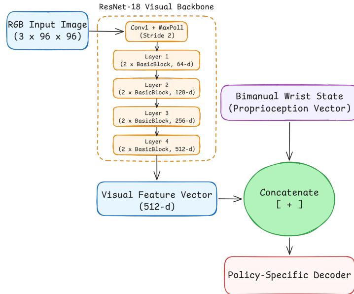
Figure 5.3 Shared ResNet-18 visual backbone preceding both policy decoders. Adapted from [57].
