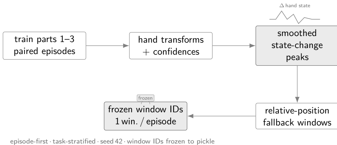
Figure 4.2 State-change-targeted sampling pipeline yielding one frozen window per episode.
