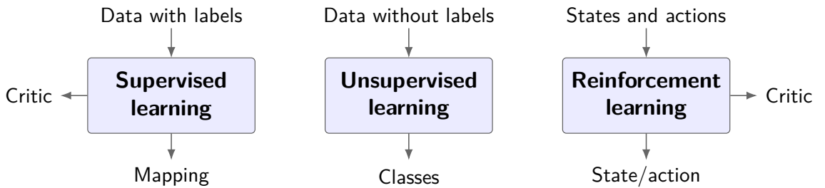
Figure 2.1 The three classical machine learning paradigms: supervised learning trains on labelled data, unsupervised learning extracts structure from unlabelled data, and reinforcement learning learns from a reward signal over states and actions [12]. SSL, central to the world models in this work, is a modern form of learning from unlabelled data in which prediction targets are constructed from the data itself [13].
