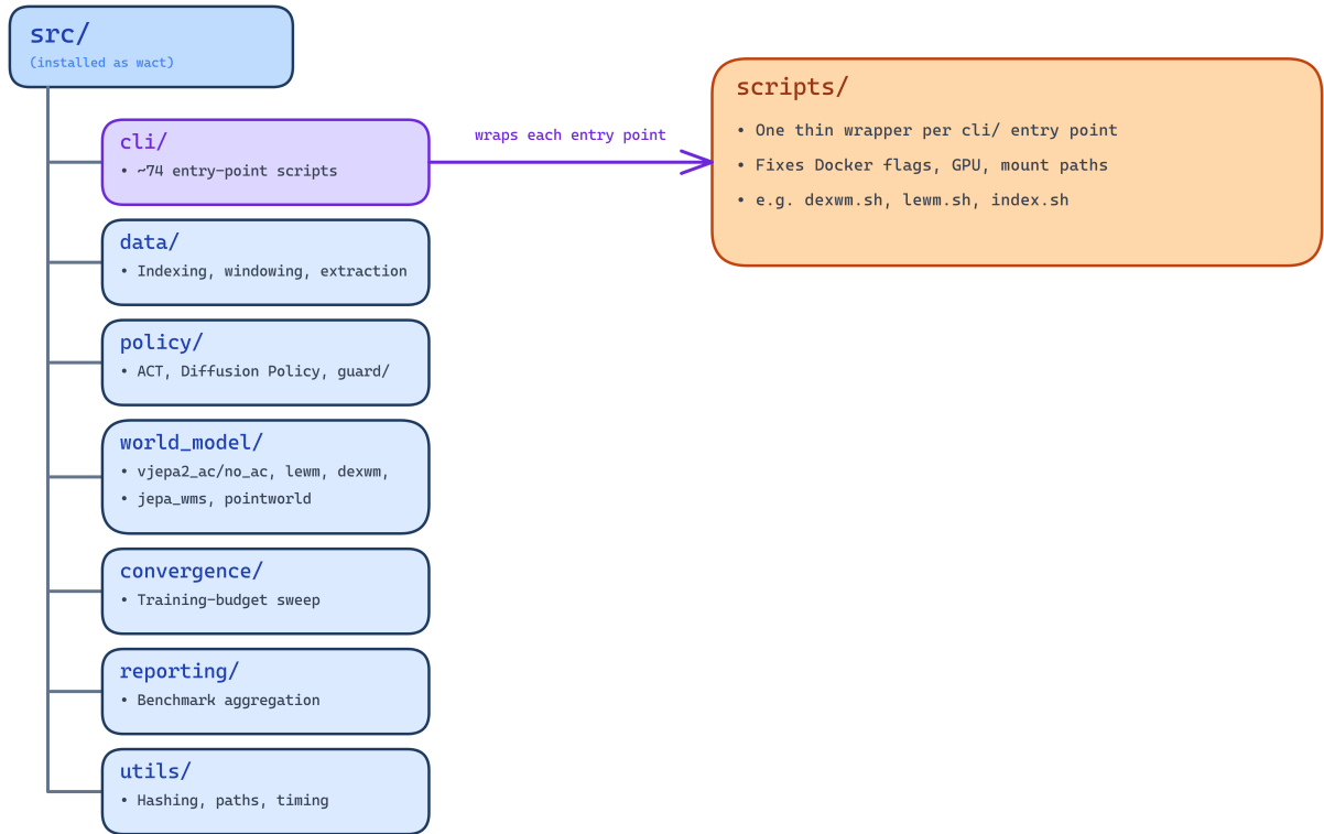
Figure 5.1 Package structure under src/ , and how scripts/ wraps each cli/ entry point. policy/guard and every world_model/ submodule implement the scoring interface used by the guard evaluation of Section 5.8.
