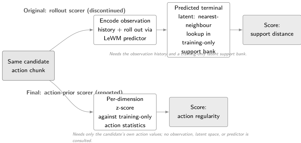
Figure 5.7 The two LeWM scoring routes implemented in this study, starting from the same candidate action chunk. The original rollout scorer (top) encodes the observation history, rolls the candidate forward through the LeWM predictor, and looks up the nearest training-only latent; the final action-prior scorer (bottom, the route reported as a result) skips visual rollout entirely and scores the candidate's own action values directly against training-only statistics.
