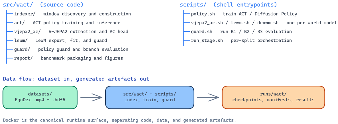
Figure 5.1 Repository structure and data flow. Source code and shell entrypoints are version-controlled; datasets and run outputs are not, keeping the audit trail between code and generated evidence unambiguous.
