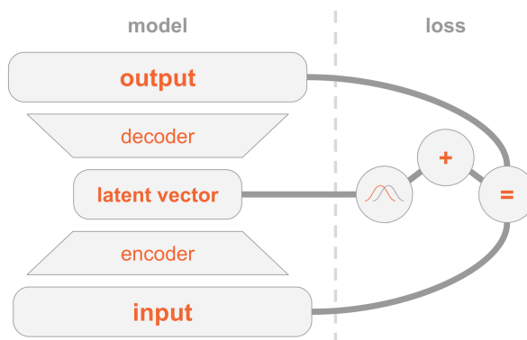
Figure 1.7 VAE encoder-decoder architecture and two-part training loss (reconstruction and regularisation) [15].
