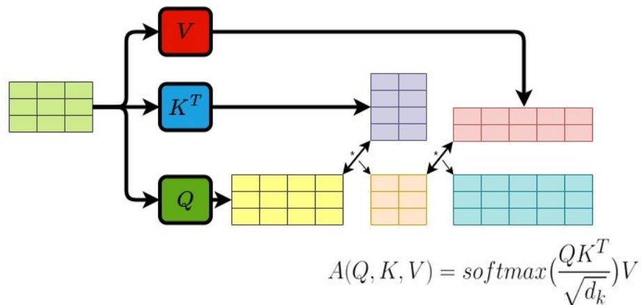
Figure 1.8 Transformer attention block: each token queries all others with Q , gathers weighted values V via keys K , and the weighted sum yields the updated output token [17].
