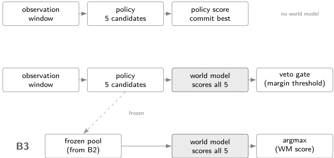
Figure 4.3 Three-branch design space. Selection authority shifts from policy alone (B1) through world-model veto (B2) to full world-model authority (B3). B3 operates over the frozen candidate pool from B2; the policy is not re-run.
