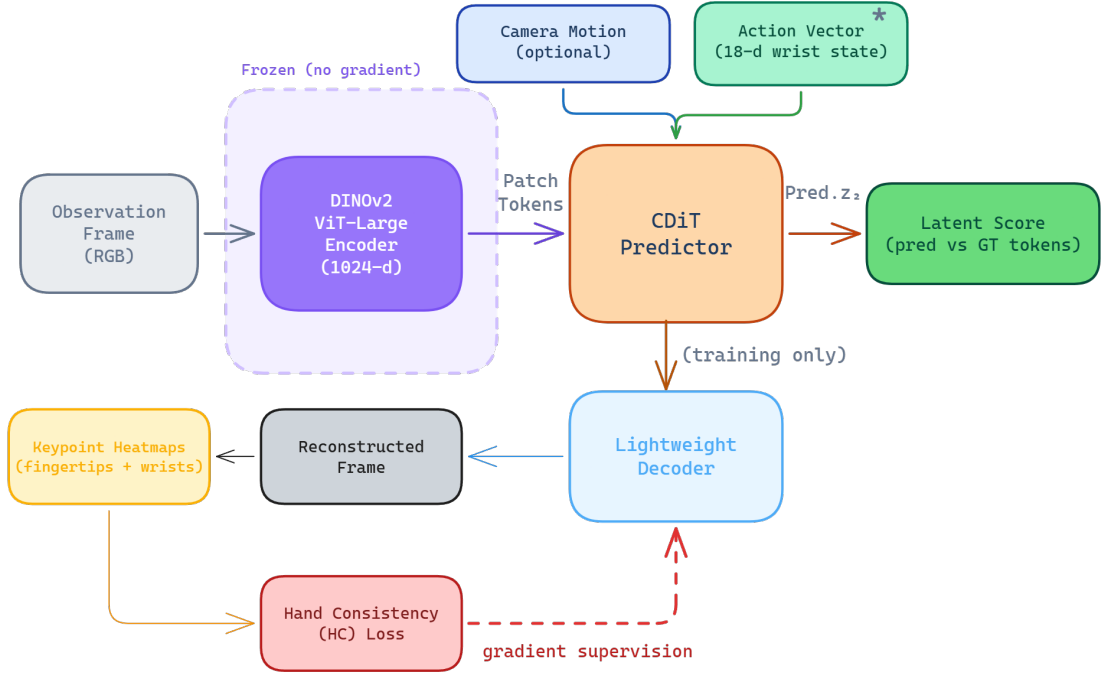
Figure 5.8 DexWM pipeline as implemented, comprising a frozen DINOv2 encoder, CDiT predictor, lightweight decoder, and HC loss supervision path. Adapted from [24].
