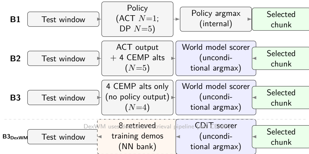
Figure 4.4 Guard evaluation pipeline for all branches. B2 pools include the ACT output alongside four CEMP-planned alternatives; B3 pools contain the four CEMP alternatives only, with the policy output excluded. The DexWM B3 variant (dashed border) uses a distinct pipeline in which eight retrieved training demonstrations replace the CEMP pool; see Section 4.8.
