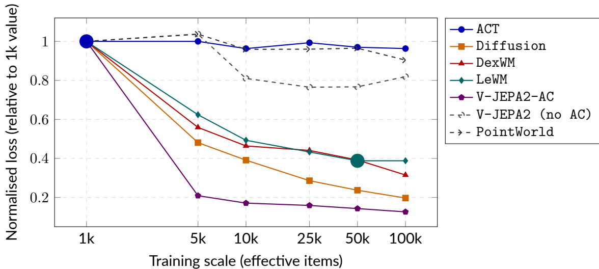
Figure 4.3 Normalised validation loss (each family’s value divided by its 1k loss) across six training scales. Solid lines are primary models; dashed lines are controls. Large filled circles mark saturation points matching the bold entries in Table 4.3. Families with no marker are still declining at 100k.
