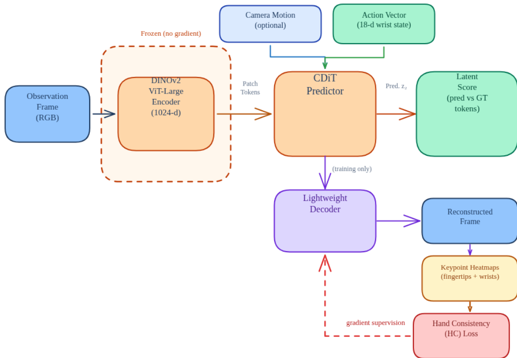
Figure 4.2 DexWM pipeline as implemented, comprising a frozen DINOv2 encoder, CDiT predictor, lightweight decoder, and HC loss supervision path. Adapted from [33].
