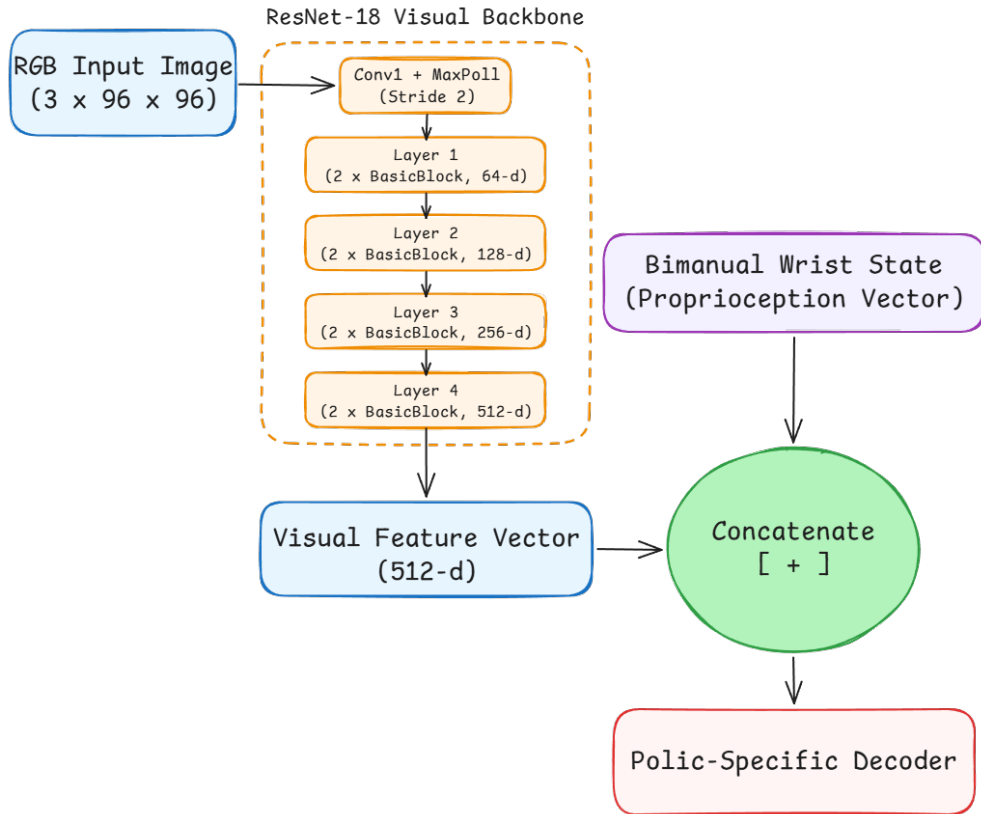
Figure 4.1 Shared ResNet-18 visual backbone preceding both policy decoders. Adapted from [50].
