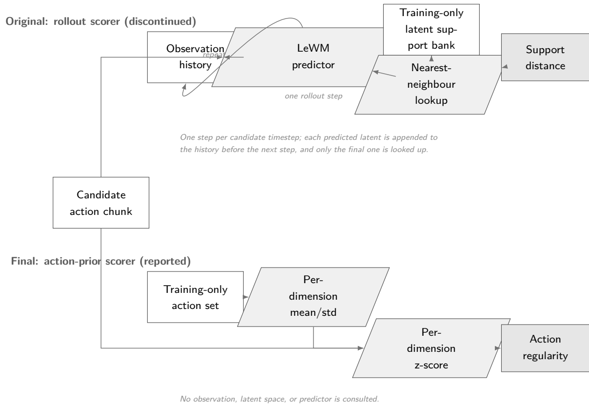
Figure 5.7 The two LeWM scoring routes implemented in this study, starting from the same candidate action chunk. The original rollout scorer (top) autoregressively rolls the candidate forward through the LeWM predictor, feeding each predicted latent back into the observation history for the next step, then looks up the final predicted latent’s nearest neighbour in a training-only latent support bank. The final action-prior scorer (bottom, the route reported as a result) skips visual rollout entirely and scores the candidate’s own action values directly against training-only action statistics.
