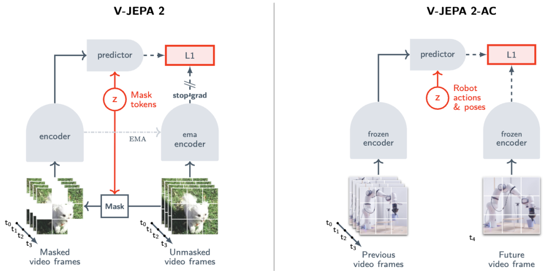
Figure 3.6 Standard V-JEPA2 (left) versus action-conditioned V-JEPA2-AC (right) [24].
