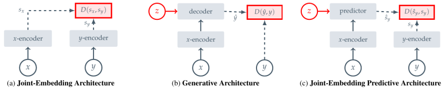
Figure 3.4 Three SSL prediction paradigms: joint-embedding (a), generative (b), and joint-embedding predictive (c) [14].
