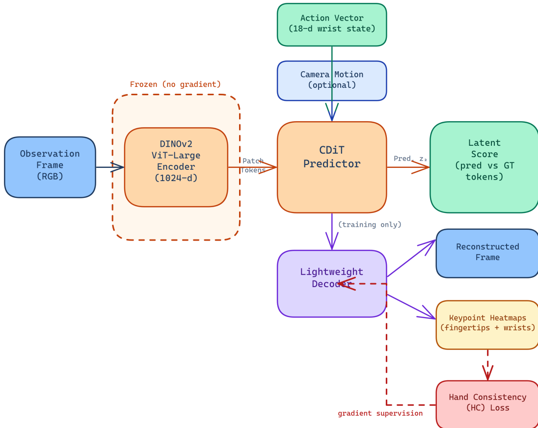
Figure 4.2 DexWM pipeline as implemented: frozen DINOv2 ViT-Large encoder producing spatial patch tokens; CDiT predictor conditioned on action and camera-motion inputs; lightweight decoder producing reconstructed frames and keypoint heatmaps; Hand Consistency (HC) loss supervising fingertip and wrist heatmap predictions during training. Latent score is computed by comparing predicted tokens against ground-truth tokens from the next frame. Adapted from [33].
