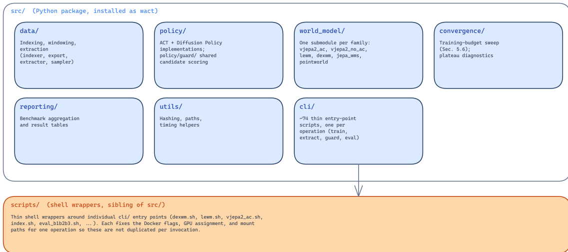
Figure 5.1 Package structure under src/ . Each module owns one concern; policy/guard and every world_model/ submodule implement the scoring interface used by the guard evaluation of Section 5.8.
