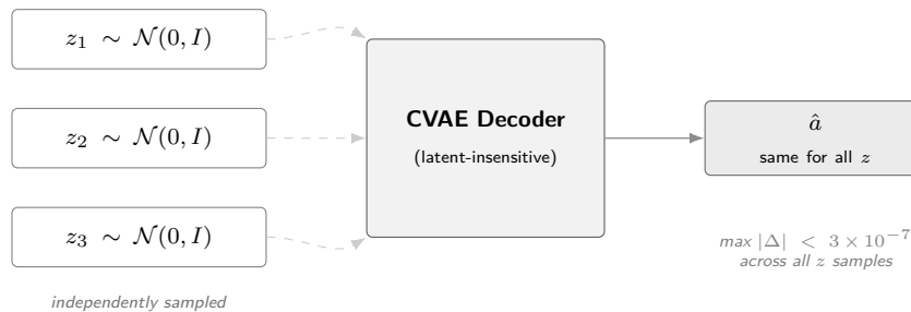
Figure 5.3 CVAE posterior collapse in the trained ACT checkpoint. Three independently sampled latent vectors z_1, z_2, z_3 are passed to the CVAE decoder (dashed arrows indicate the latent path the decoder effectively ignores). All inputs produce an identical output \hat{a} ; the decoder has learned to reconstruct the action from the visual observation alone, making the latent redundant.
