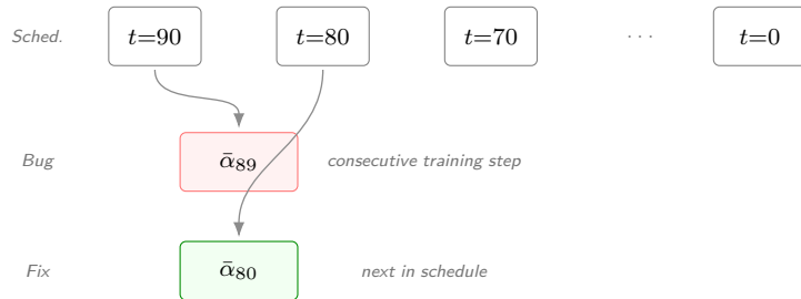
Figure 5.5 DDIM subsampling correction. The ten-step inference schedule spans t \in \{90, 80, \dots, 0\} . At each reverse step the correct \bar{\alpha}_{t_{\text{prev}}} is the next timestep in the subsampled schedule ; the bug substituted the consecutive training-schedule timestep \bar{\alpha}_{t-1} , miscalibrating the \hat{x}_0 weighting at every step.
