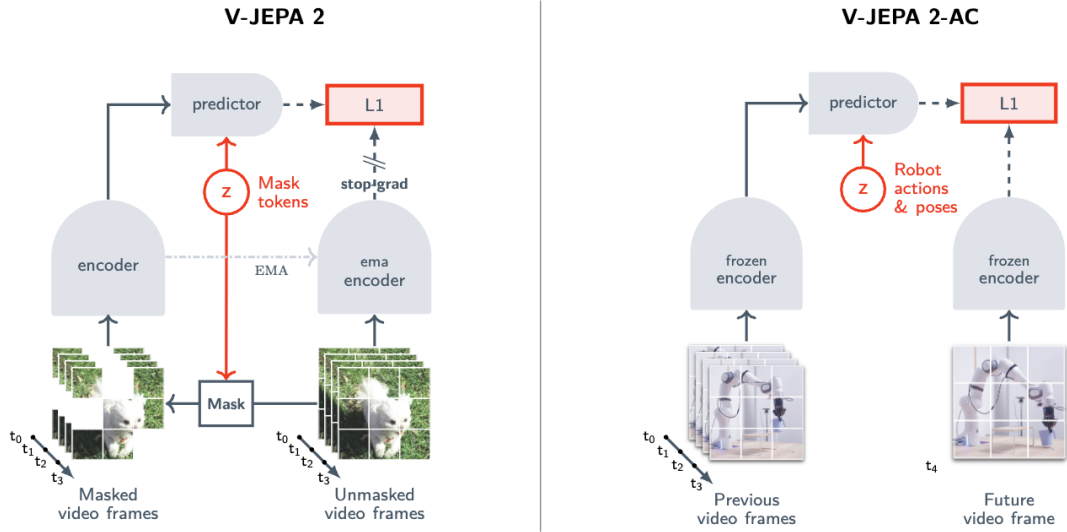
Figure 3.8 Standard V-JEPA2 (left) versus action-conditioned V-JEPA2-AC (right) [23].
