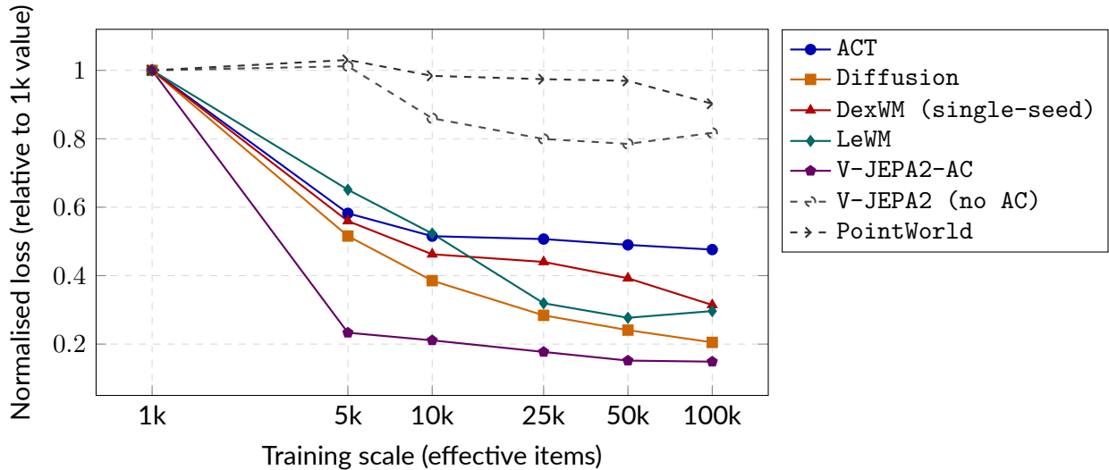
Figure B.1 Normalised validation loss (each family's value divided by its 1k loss) across six training scales, pooled across 3 seeds except DexWM (single-seed). Solid lines are primary models; dashed lines are controls. No family shows a clean saturation point once pooled (the discussion above explains why ACT and LeWM appeared to in an earlier single-seed reading), so no saturation markers are shown; every family is still declining, or in LeWM's case turning slightly upward, at 100k.
