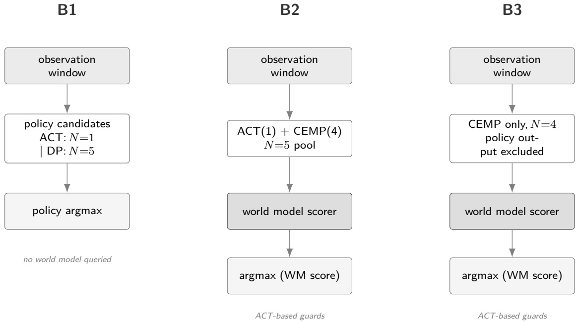
Figure 3.3 Three-branch evaluation framework. B1 selects from the policy’s own candidate output. B2 and B3 introduce world-model scoring over a CEMP-generated pool; B3 additionally excludes the policy’s own output, leaving the world model to choose among planned alternatives only.
