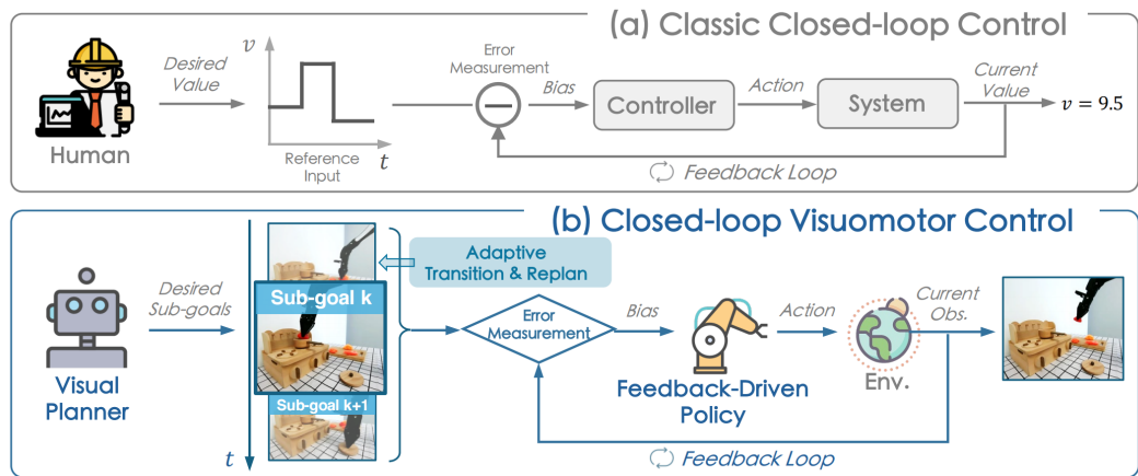
Figure 3.3 Classic closed-loop control (a) versus CLOVER’s closed-loop visuomotor control (b) [32].
