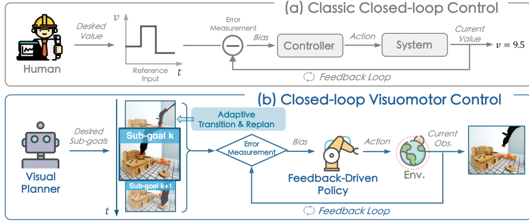
Figure 3.3 Classic closed-loop control (a) versus CLOVER’s closed-loop visuomotor control (b) [36].
