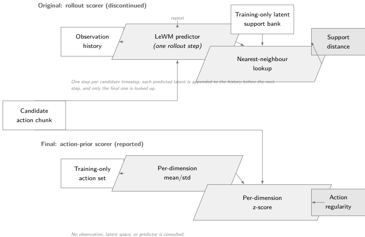
Figure 5.7 The two LeWM scoring routes implemented in this study, starting from the same candidate action chunk. The original rollout scorer (top) autoregressively rolls the candidate forward through the LeWM predictor, feeding each predicted latent back into the observation history for the next step, then looks up the final predicted latent’s nearest neighbour in a training-only latent support bank. The final action-prior scorer (bottom, the route reported as a result) skips visual rollout entirely and scores the candidate’s own action values directly against training-only action statistics.
