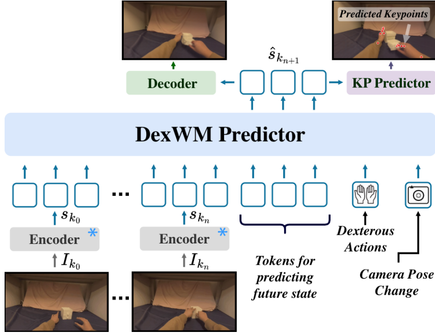
Figure 3.7 DexWM world model pipeline [34].
