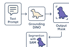
Figure 1: Prompt-conditioned grounding: open-set detectors require a text prompt before localisation can begin.
