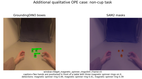
Figure 7: Additional qualitative Object Pose Estimation (OPE) pipeline example from a ring handling episode, included to show a second object configuration beyond the cup dominated case.
