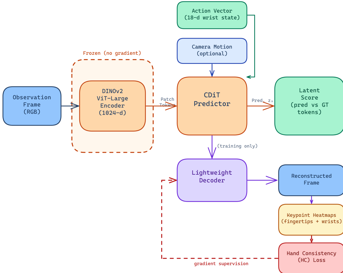
Figure 4.2 DexWM pipeline as implemented, comprising a frozen DINOv2 encoder, CDiT predictor, lightweight decoder, and HC loss supervision path. Adapted from [33].
