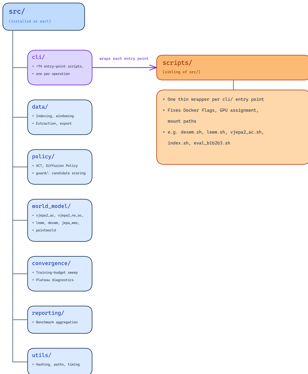
Figure 5.1 Package structure under src/ , and how scripts/ wraps each cli/ entry point. policy/guard and every world_model/ submodule implement the scoring interface used by the guard evaluation of Section 5.8.
