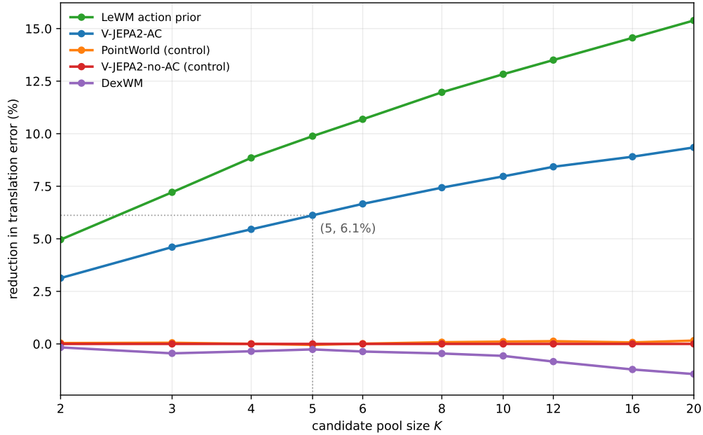
Figure B.3 Reduction in translation error against candidate pool size for the five world-model scorers on the Diffusion Policy row. All points are scored on nested pools, so differences along a curve reflect pool size alone. Pooled across 3 seeds except DexWM, which remains single-seed (Section 4.7). The vertical guide marks the operating point used throughout this dissertation.
