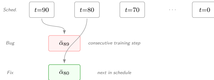
Figure 5.5 DDIM subsampling correction. The ten-step inference schedule spans t \in \{90, 80, \dots, 0\} . At each reverse step the correct \bar{\alpha}_{t_{\text{prev}}} is the next timestep in the subsampled schedule ; the bug substituted the consecutive training-schedule timestep \bar{\alpha}_{t-1} , miscalibrating the \hat{x}_0 weighting at every step.
