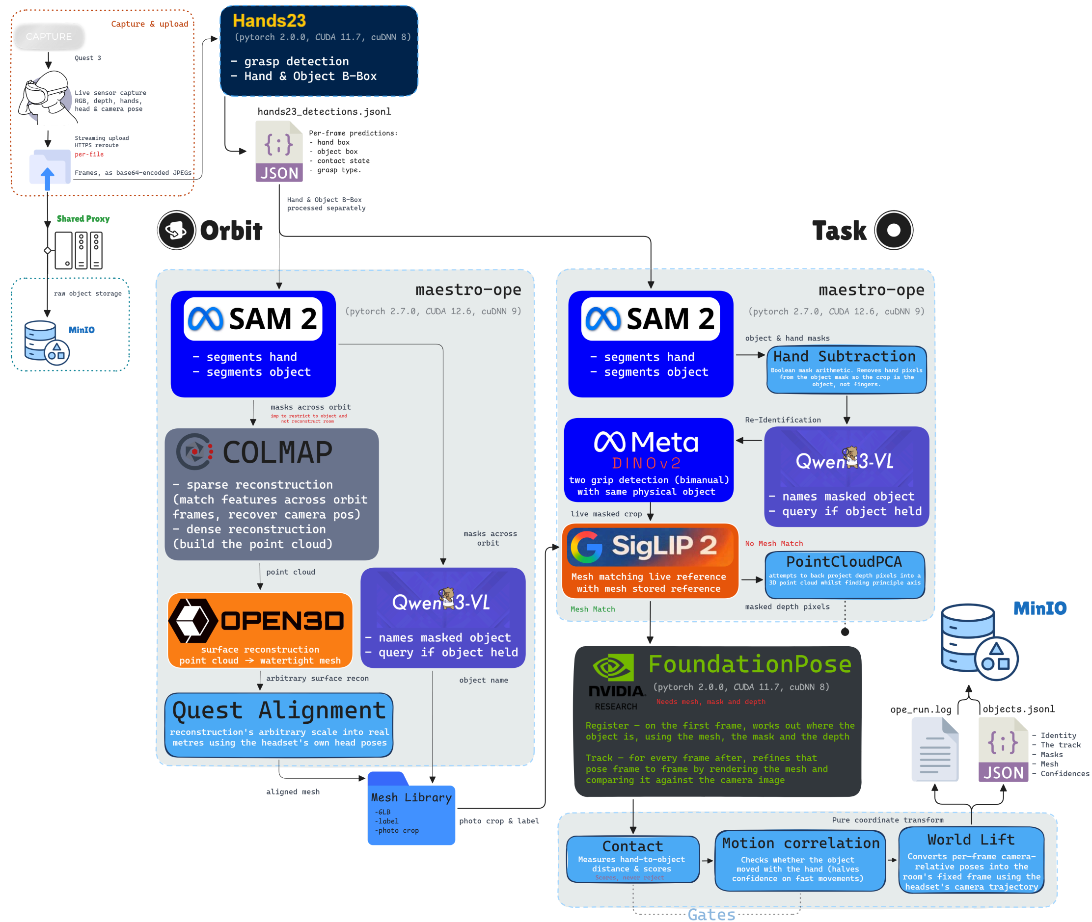
Figure 1. Maestro VR pipeline, preserved from the supplied audit assets. Arrows describe architectural relationships, including conditional and disabled paths. The October 3 hand-distance guard is documented below and is not drawn in this earlier diagram.
