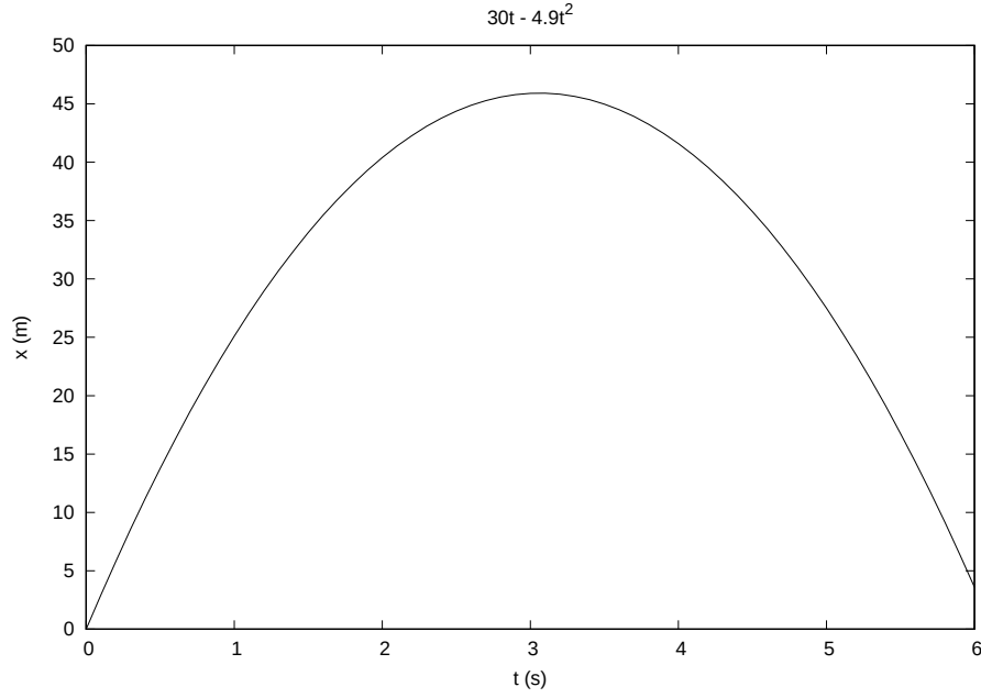
Figure 11.3: Plot of x(t) = 30t - 4.9t^2
