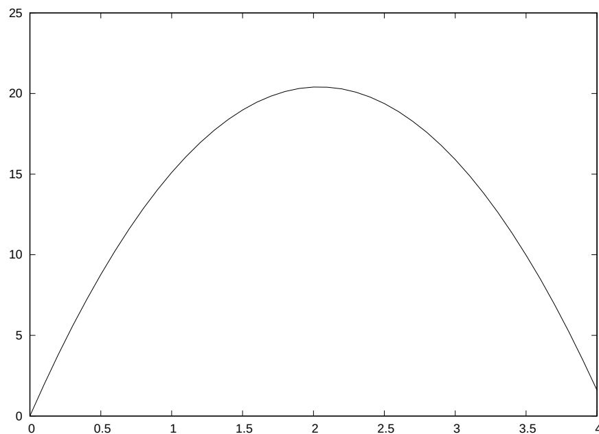
Figure 7.3: Plot of yRock20 function from t = 0 to t = 4s
