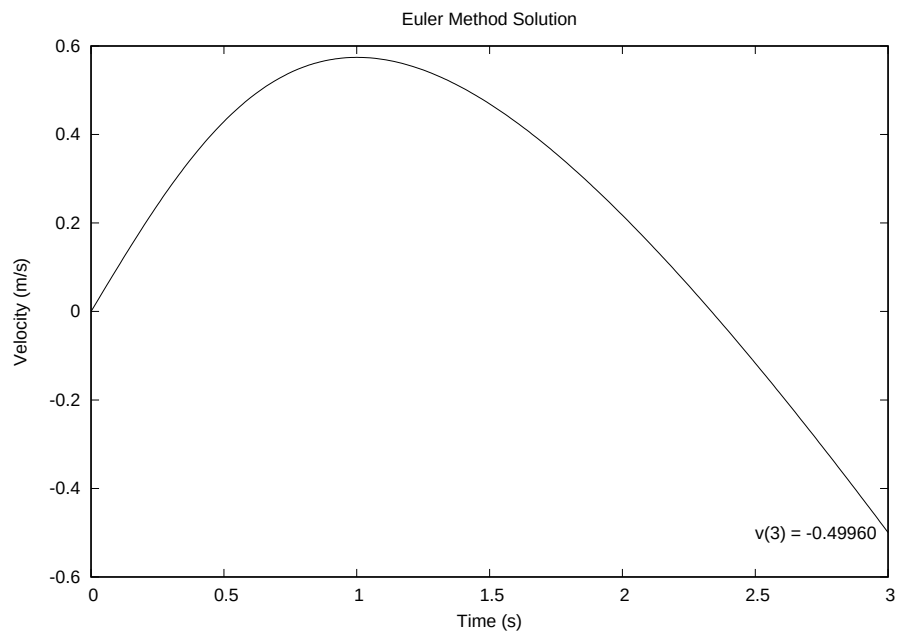
Figure 14.4: Euler method solution to differential equation
