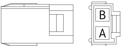
LT_UTIL_FLR_O_LP_UTIL_2A 23-13141-200
