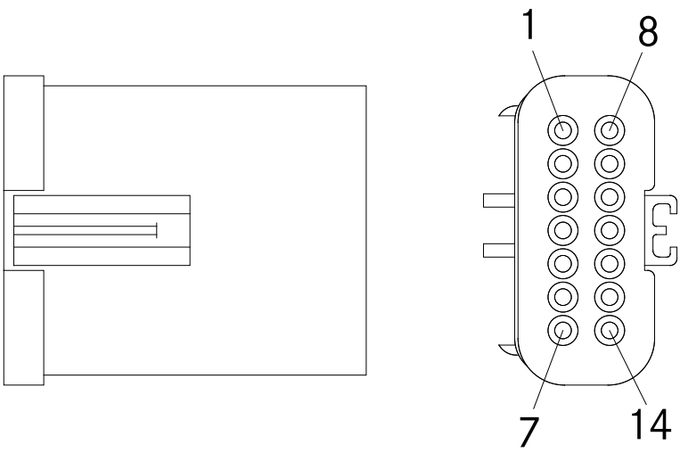
FLR_H_DASH_RH_CBR_2B ⓘ (INTEGRATED SEALS) 23-13153-012
