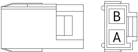
LT_UTIL_FLR_O_LP_UTIL_1A 23-13141-200
