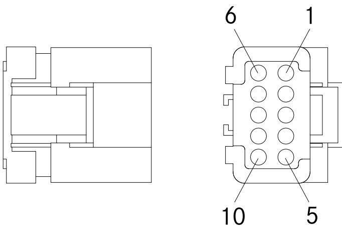
LT_HDLP_CHAS_F_O_LP_HDLP_LED_LH_1A (INTEGRATED SEALS) 23-13153-003
