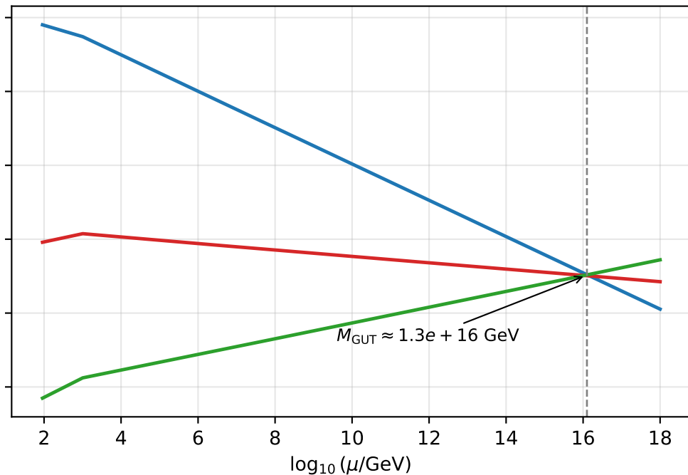
MSSM ( m_{\text{SUSY}} = 1000 \text{ GeV} ): unification
