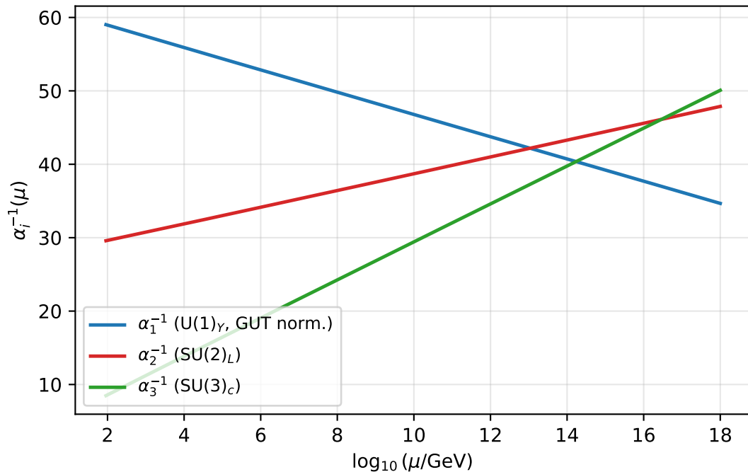
Standard Model: near miss
