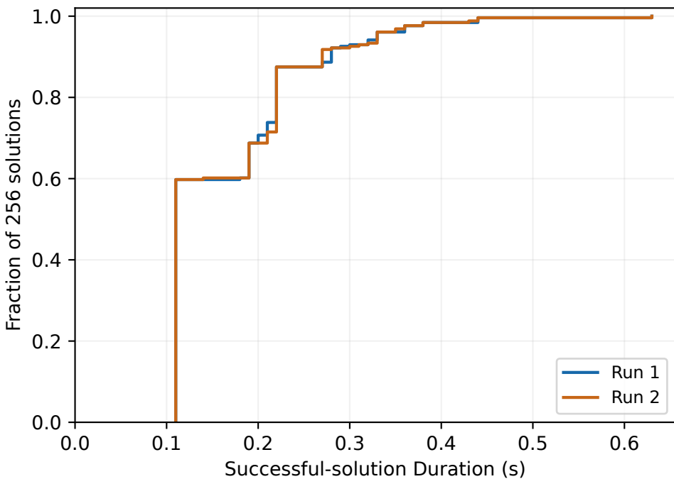
EvolveNew
